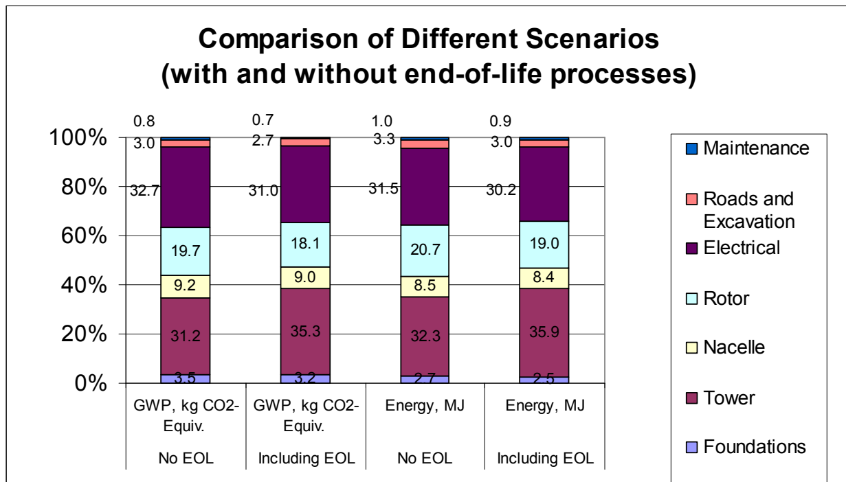
Figure 4: Comparison of the relative impact of each component of the proposed Hauāuru mā raki Wind Farm with and without end-of-life taken into account
