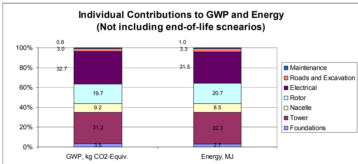
Figure 3: GHG emissions and primary energy use of proposed Hauāuru mā raki Wind Farm over its whole life cycle in % of the total
