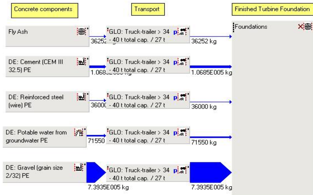
Figure 1: GaBi model of foundation used in proposed Hauāuru mā raki Wind Farm
