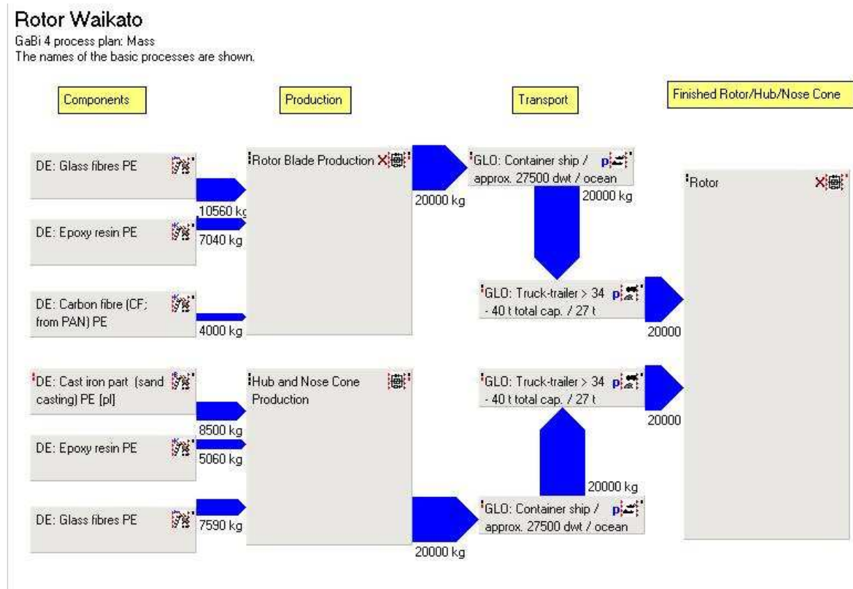
Figure 2: GaBi model of the rotor system at the proposed Hauāuru mā raki Wind Farm (one turbine)
